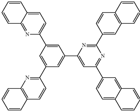
[Chemical Formula 37]
