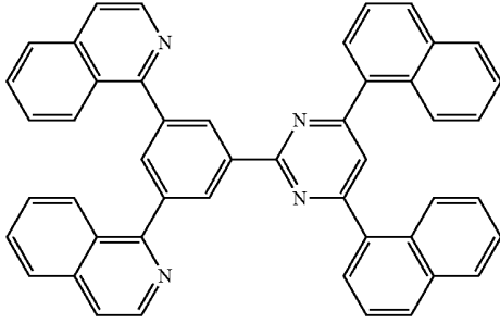
[Chemical Formula 22]
