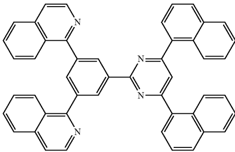
[Chemical Formula 21]
