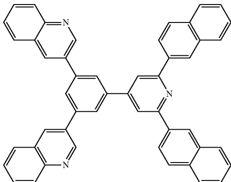
[Chemical Formula 34]
