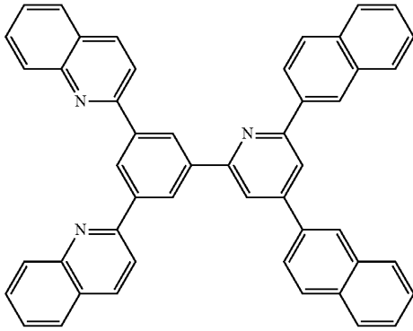
[Chemical Formula 39]
