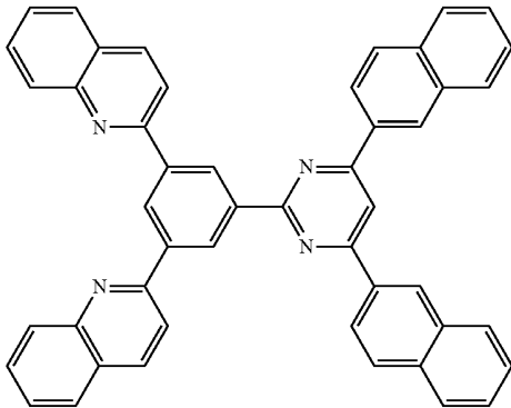
[Chemical Formula 40]
