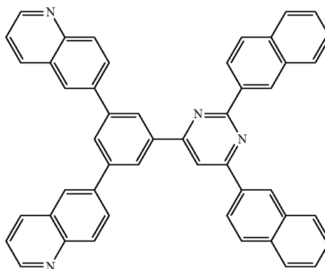
[Chemical Formula 45]
