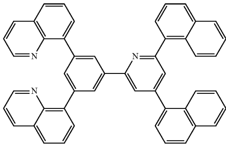
[Chemical Formula 49]
