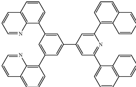
[Chemical Formula 48]
