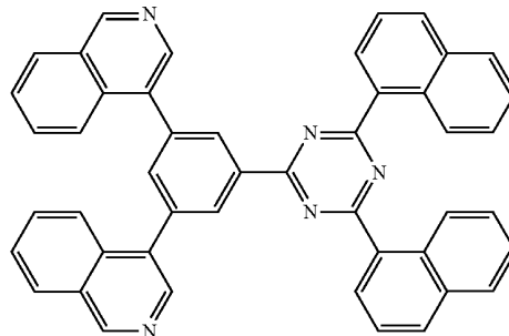
[Chemical Formula 27]
