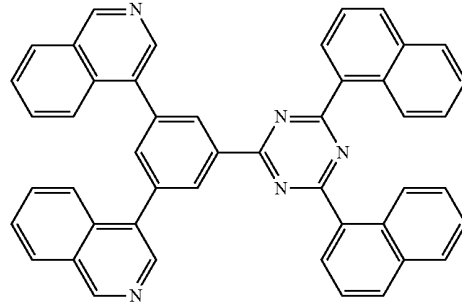
[Chemical Formula 30]
