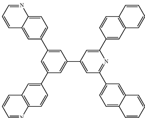
[Chemical Formula 44]
