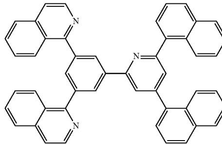
[Chemical Formula 19]
