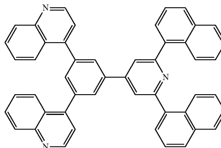
[Chemical Formula 43]
