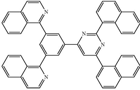
[Chemical Formula 21]
