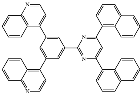
[Chemical Formula 42]
