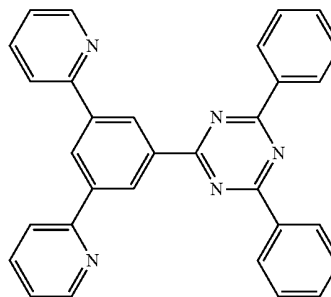
[Chemical Formula 3]
