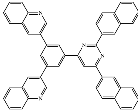
[Chemical Formula 32]
