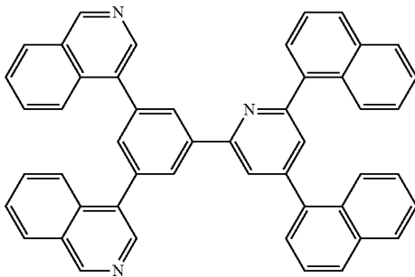
[Chemical Formula 29]
