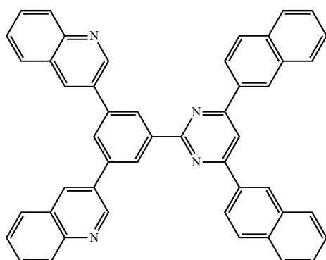
[Chemical Formula 30]
