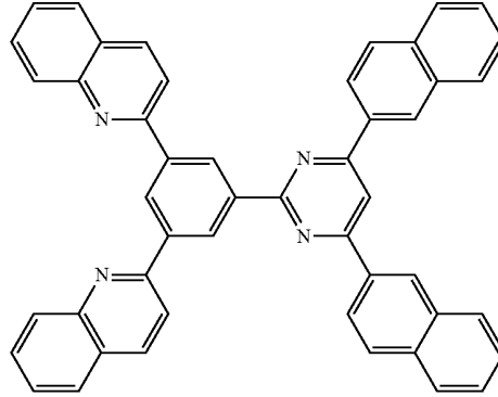
[Chemical Formula 38]
