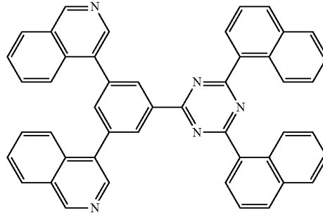
[Chemical Formula 30]
