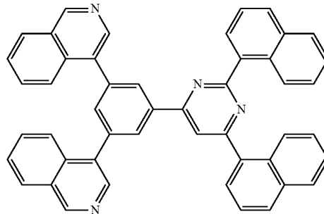
[Chemical Formula 26]
