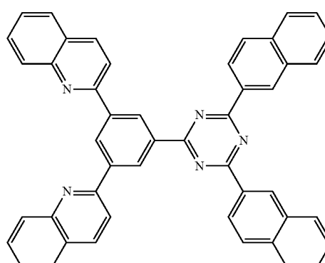
[Chemical Formula 33]
