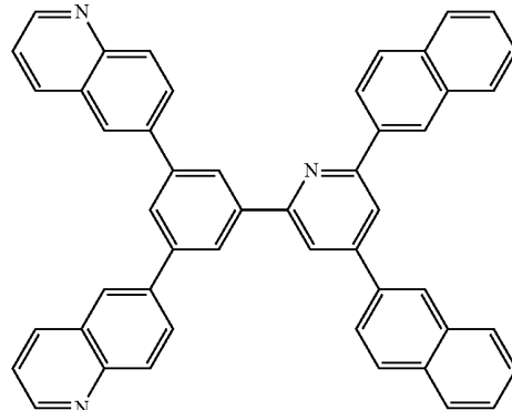
[Chemical Formula 49]
