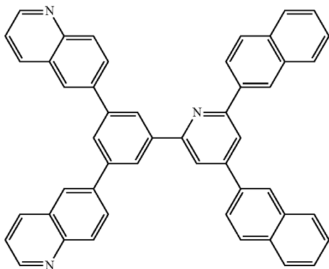
[Chemical Formula 44]
