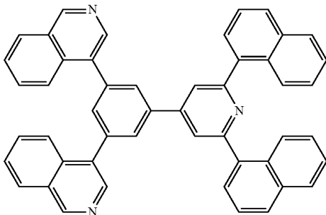
[Chemical Formula 23]
