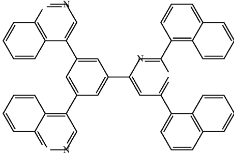
[Chemical Formula 29]
