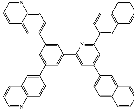
[Chemical Formula 44]
