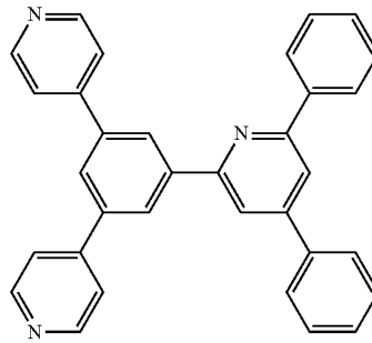
[Chemical Formula 10]
