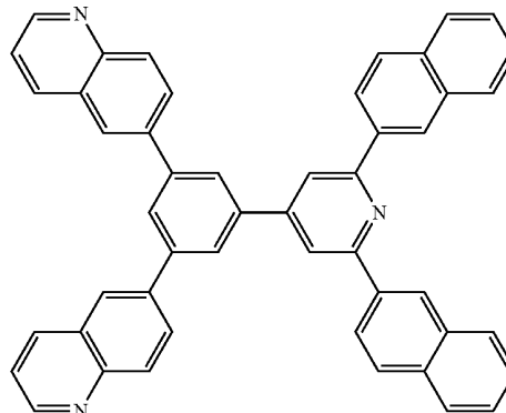
[Chemical Formula 48]
