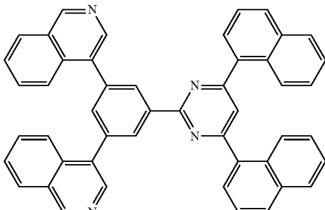
[Chemical Formula 26]
