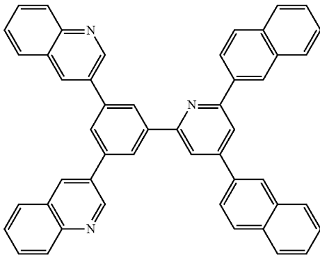
[Chemical Formula 35]
