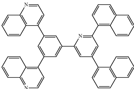
[Chemical Formula 39]
