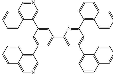
[Chemical Formula 25]
