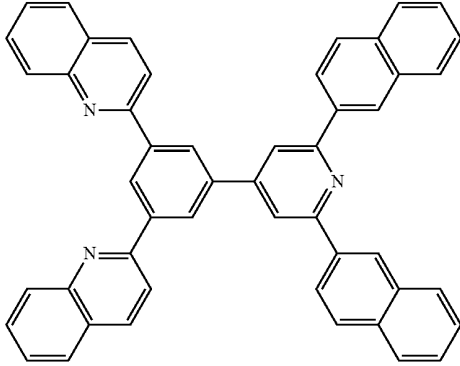
[Chemical Formula 34]
