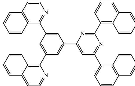
[Chemical Formula 20]
