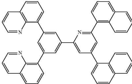
[Chemical Formula 49]
