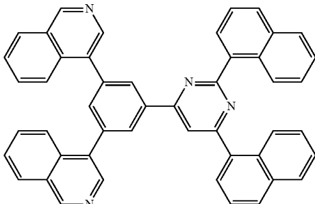
[Chemical Formula 25]
