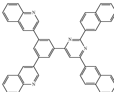
[Chemical Formula 31]
