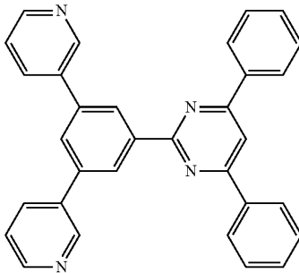
[Chemical Formula 6]
