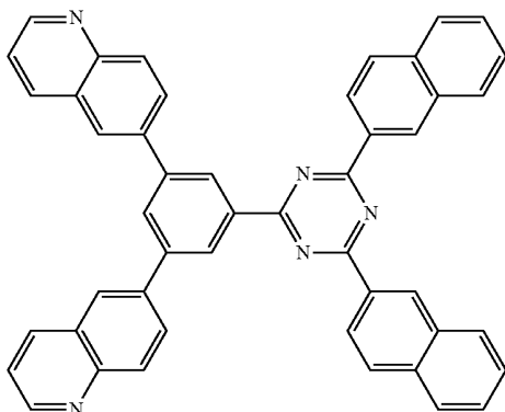
[Chemical Formula 50]
