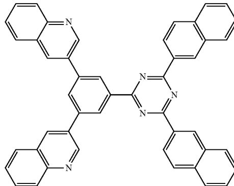
[Chemical Formula 32]
