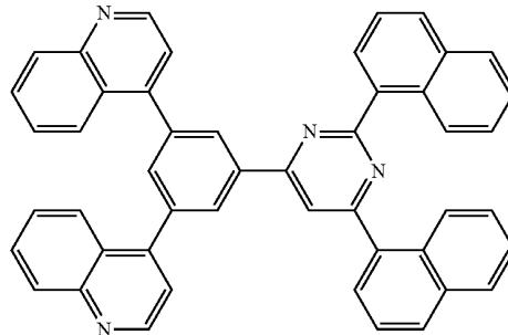
[Chemical Formula 40]
