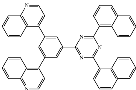
[Chemical Formula 43]
