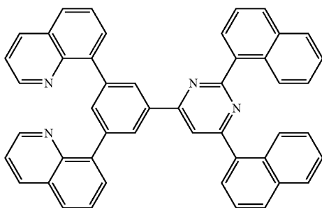
[Chemical Formula 51]
