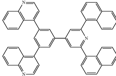
[Chemical Formula 39]
