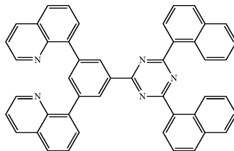
[Chemical Formula 52]
