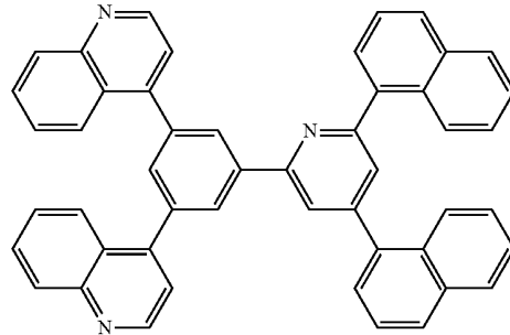
[Chemical Formula 44]
