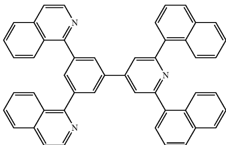
[Chemical Formula 23]
