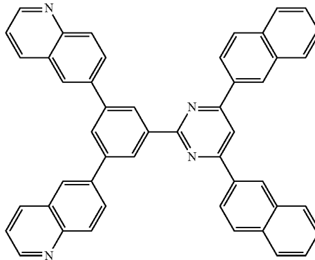
[Chemical Formula 46]
