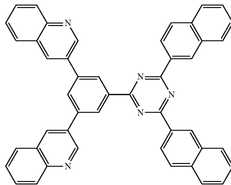
[Chemical Formula 32]
