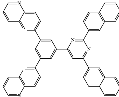
[Chemical Formula 46]
