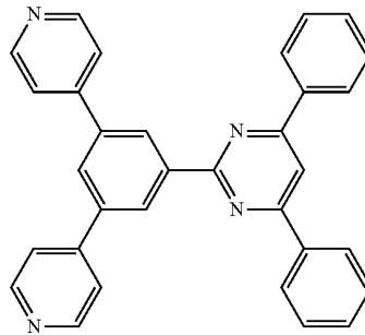
[Chemical Formula 11]
