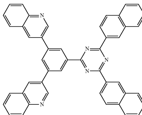
[Chemical Formula 32]
