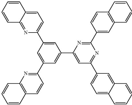
[Chemical Formula 36]
