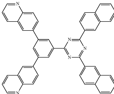
[Chemical Formula 47]
