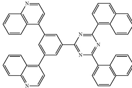
[Chemical Formula 45]
