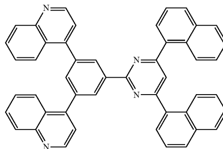
[Chemical Formula 42]
