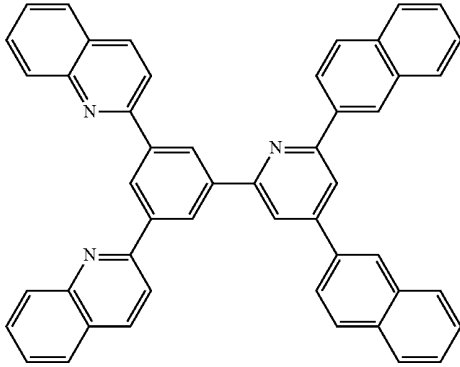
[Chemical Formula 35]
