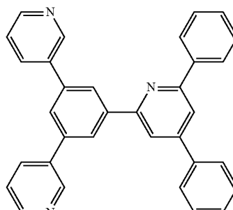
[Chemical Formula 5]
