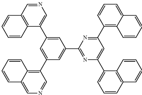
[Chemical Formula 26]
