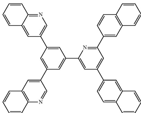
[Chemical Formula 29]
