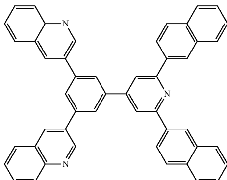
[Chemical Formula 28]
