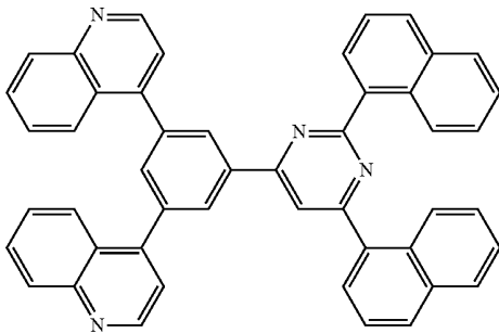
[Chemical Formula 40]
