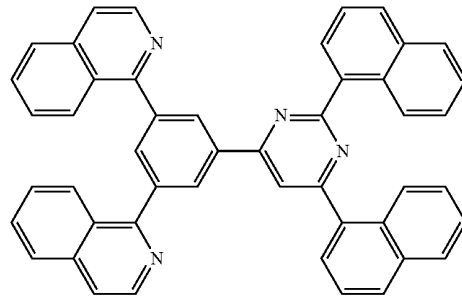
[Chemical Formula 20]
