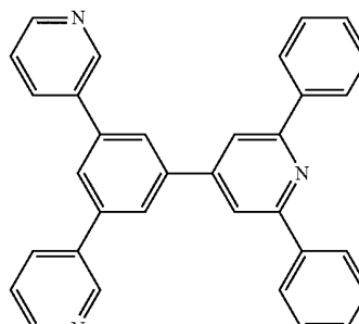
[Chemical Formula 4]
