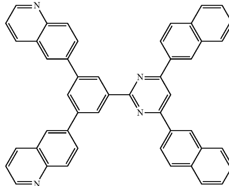
[Chemical Formula 46]
