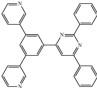
[Chemical Formula 7]
