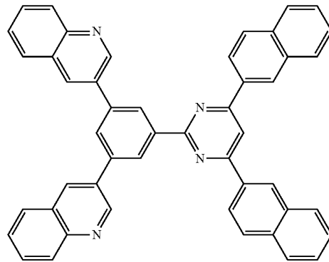
[Chemical Formula 31]
