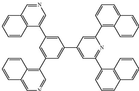
[Chemical Formula 28]
