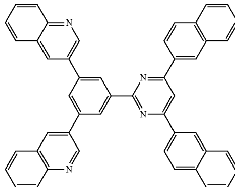
[Chemical Formula 31]
